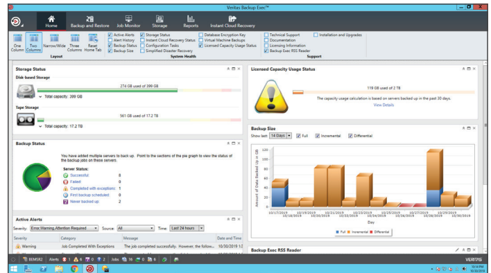
Figure 2. Backup Exec 20.6
