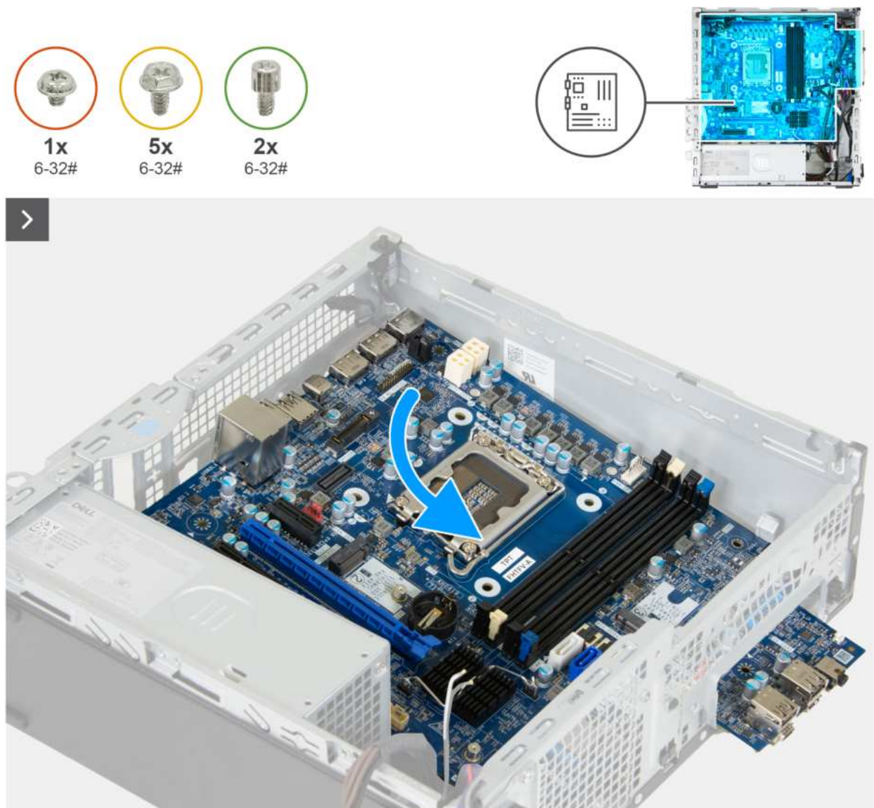
Figure 92. Installing the system board
