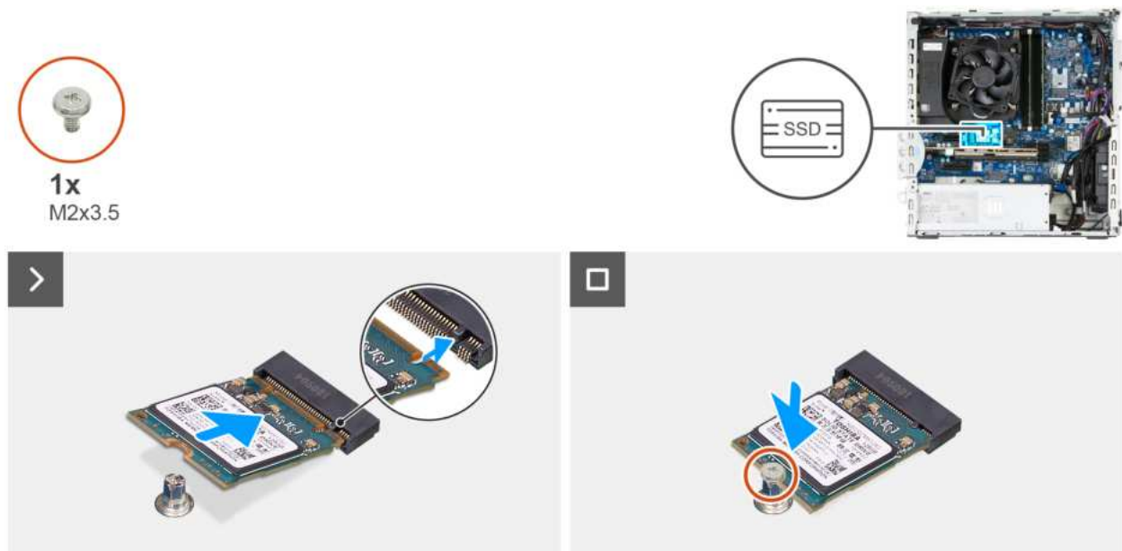
Figure 28. Installing the M.2 2230 solid state drive in slot 1
