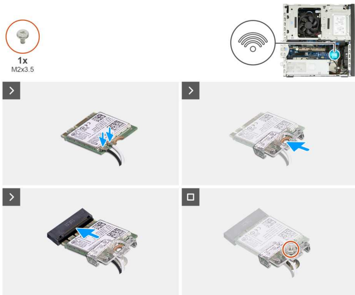
Figure 36. Installing the wireless card
