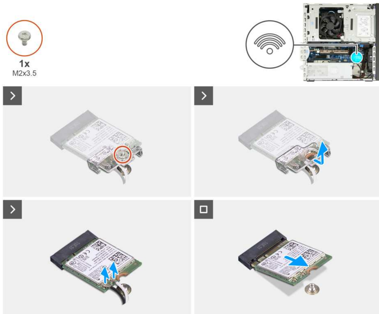
Figure 35. Removing the wireless card
