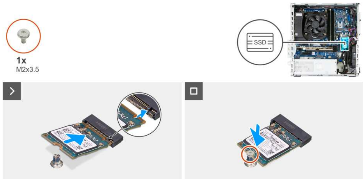
Figure 23. Installing the M.2 2230 solid state drive in slot 0
