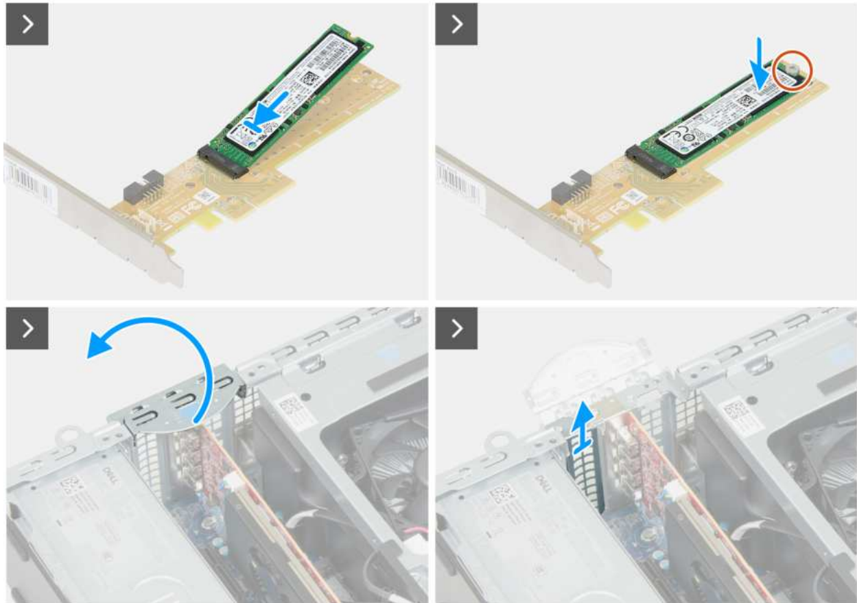
Figure 39. Installing the solid state drive expansion card
